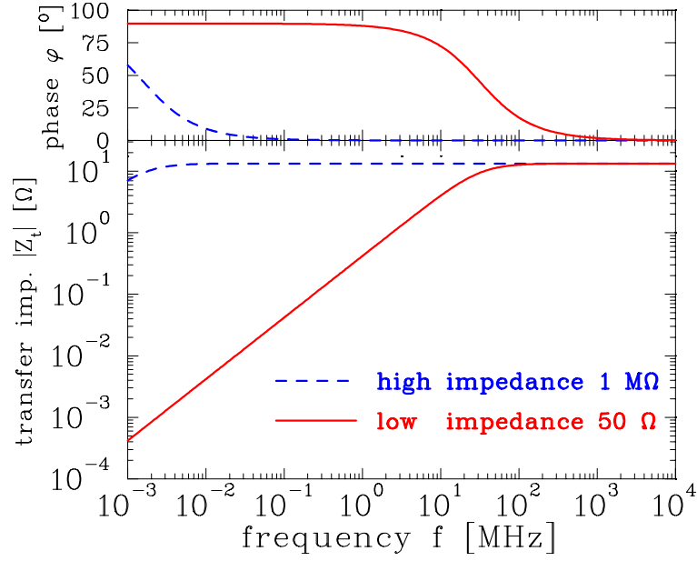
Figure 5.3: Absolute value and phase of the transfer impedance for a l = 10 cm long round pick-up with a capacitance of C = 100 pF and an ion velocity of \beta = 50\% for high ( 1 \text{ M}\Omega ) and low ( 50 \Omega ) input impedance of the amplifier. The parameters are typical for a proton/heavy ion synchrotron. The high-pass characteristic is clearly seen corresponding to a signal decreasing for low frequencies.
