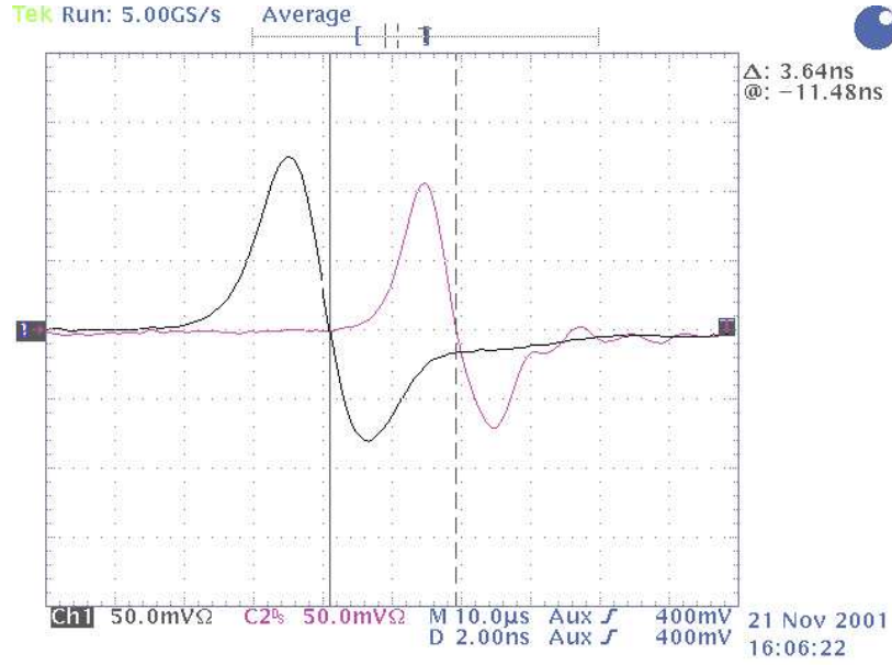
Figure 6.5: Time-of-flight signal from two pick-ups with 1.4 MeV/u at the GSI-LINAC.
