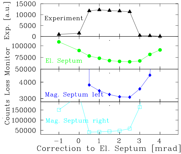
Figure 8.10: Counts per spill from three loss monitor locations and the current at the experiment as a function of the angle electrostatic septum at the GSI synchrotron [118].
