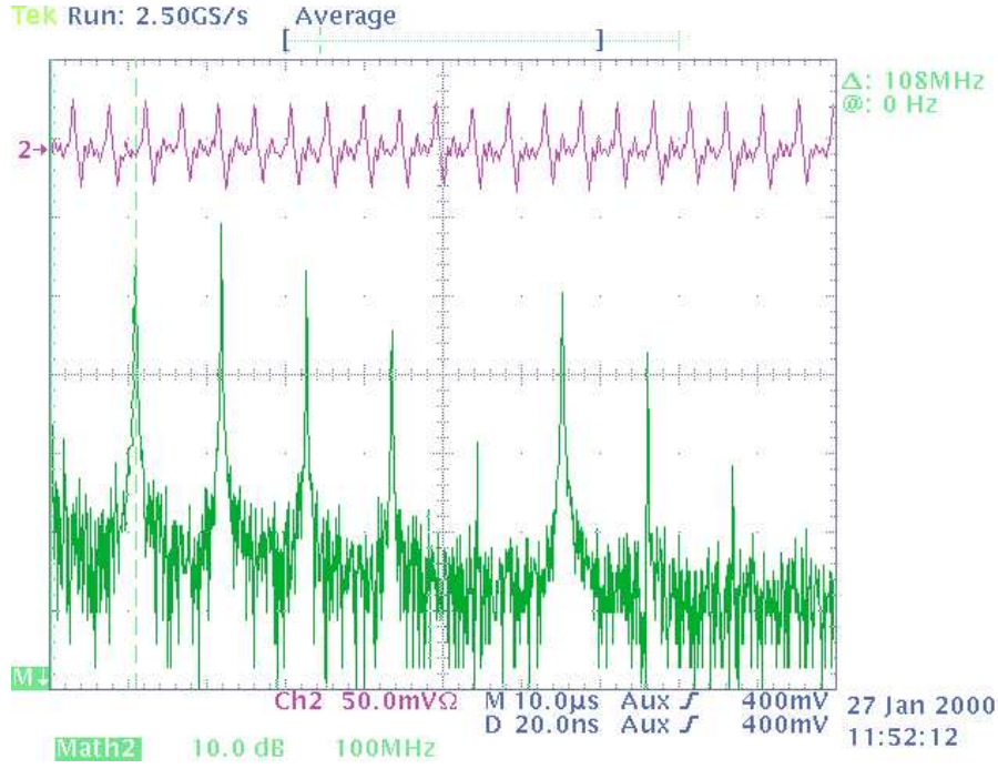
Figure 5.22: Bunch signal (top) and its Fourier components (bottom). In the Fourier spectrum each line corresponds to one harmonic of the 108 MHz accelerating frequency.
