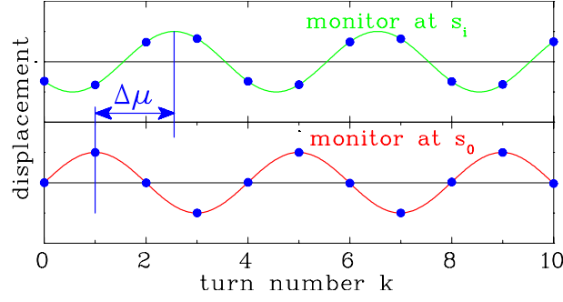
Figure 5.31: Scheme of the individual measurements at two pick-ups for a phase advance \Delta\mu determination. A sine function can be fitted through the data points.
