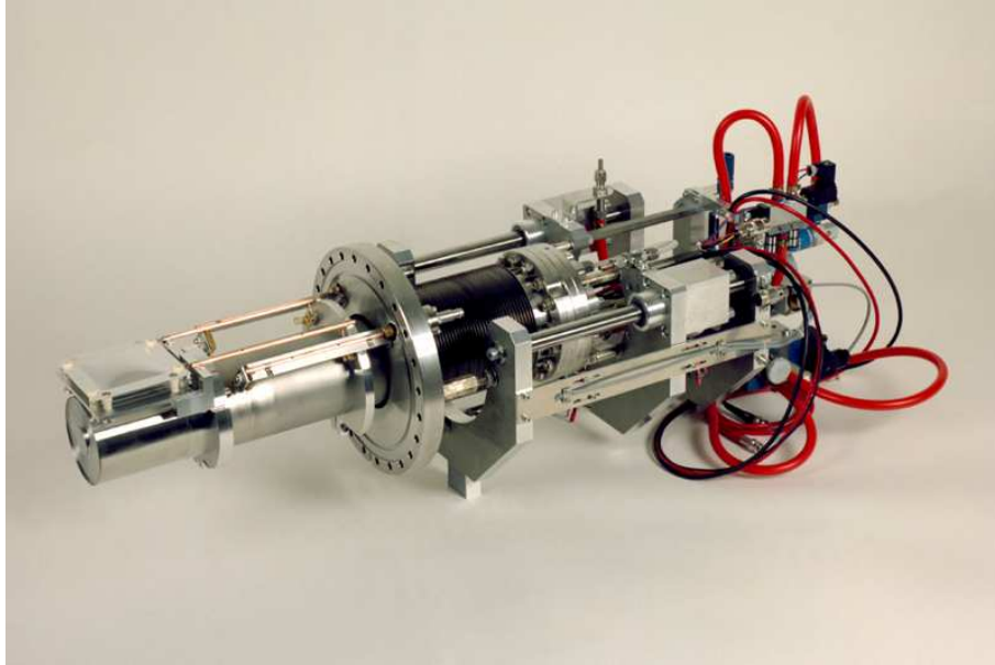
Figure 2.33: The feed-through mounted on a Ø200 mm flange containing the scintillator and IC inside the pocket at atmospheric pressure and the SEM in the vacuum.
