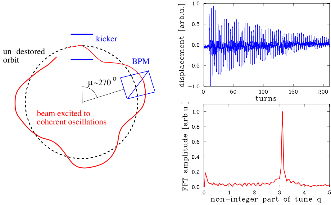
Figure 5.26: Beam oscillations after a kick excitation recorded in the time domain for 200 turns (top) and its Fourier transformation for q determination (bottom) at the GSI synchrotron.
