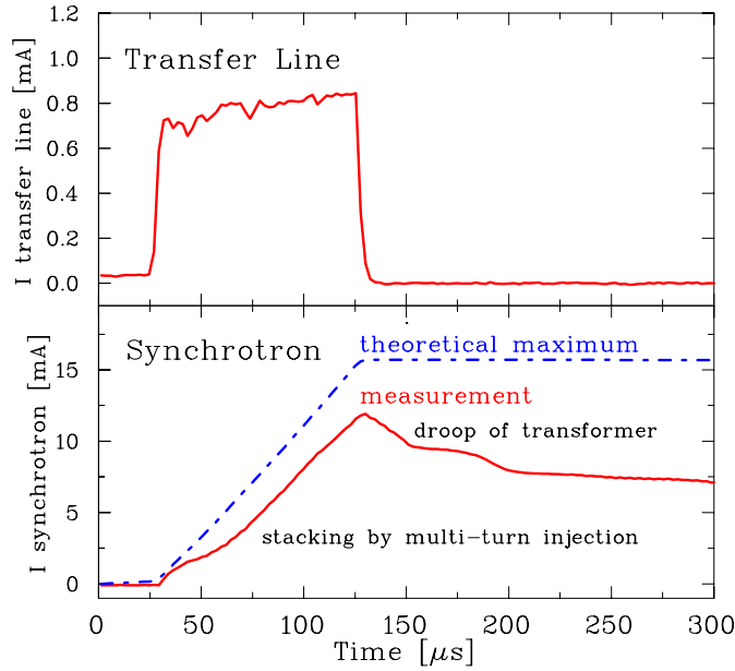
Figure 2.11: The multi-turn injection at GSI measured with two ac-transformers. The upper curve is the current delivered by the LINAC and the lower curve is the stored current in the synchrotron. In this case 20 turns are used and 70 % efficiency is reached for this \text{Ni}^{26+} beam.
