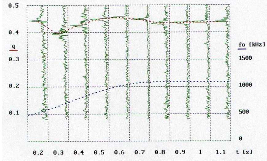
Figure 5.30: Measurement of the vertical tune at the COSY proton synchrotron [89]. Displayed is the Fourier transformation of a bunch synchronous sampling for different times (horizontal axis) during one acceleration. The maxima of the FFT are shown together with the magnetic ramp in blue.
