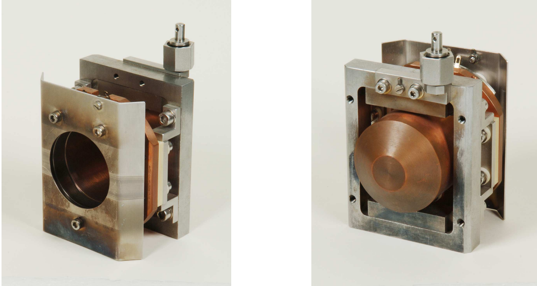
Figure 2.18: Photo of an Ø50 mm uncooled Faraday cup with magnetic and electric secondary electron suppression.
