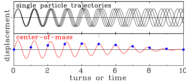
Figure 5.27: Plot of the individual trajectories of four particles after a kick (top) and the resulting coherent sum signal as measured by a pick-up (bottom). (The tune spread is much too large for a real machine.)
