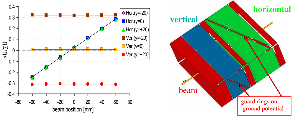
Figure 5.15: Numerical calculation of the position reading \Delta U/\Sigma U as a function of beam displacement for the horizontal plane. The plot also includes the calculations for a beam offset in the vertical direction and proves the decoupling of both planes [77]. It is performed for the pick-up shown right and in Fig 5.14 with a 200 \times 70 \text{ mm}^2 cross section and 350 mm length.
