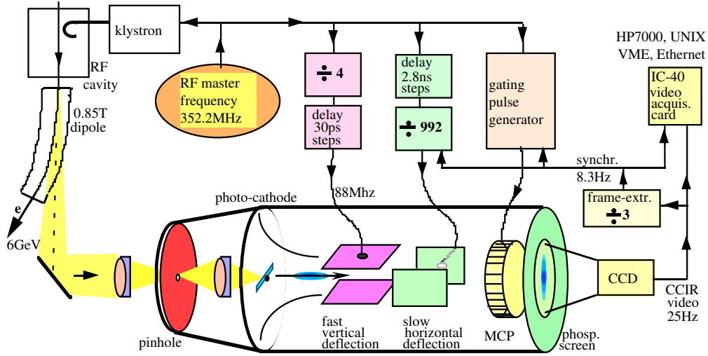
Figure 6.25: Principle of a streak camera measurement for bunch width determination at electron accelerators (here ESRF), from [105].
