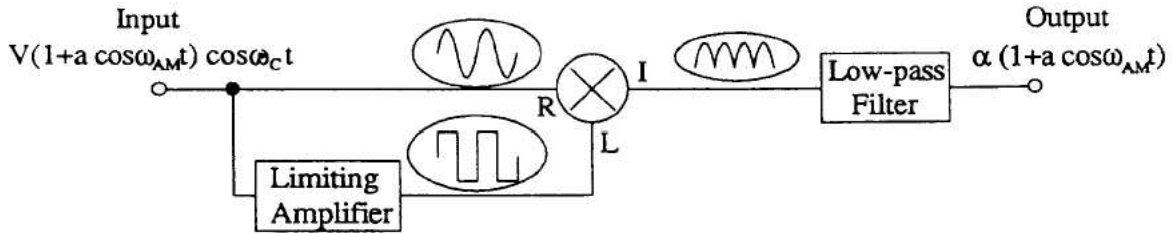
Figure 5.23: Scheme of a synchronous detector to rectify an rf signal: The rf signal is split and one branch is fed into a limiter amplifier driven into saturation, which transforms the signal to a bipolar rectangular pulse. This signal is mixed with the original signal to yield a unipolar waveform (corresponding to the square). It is passed through a low-pass filter and can then be digitized by a (slow) ADC.
