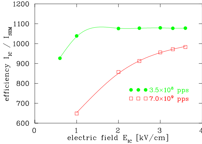
Figure 2.36: The characteristic line for the IC as determined of the 300 MeV/u \text{Ne}^{10+} beam. The efficiency, as measured by the ratio of the secondary current of the IC and the SEM as a function of the applied electric field [16]. For low primary current a plateau is reached, while for a high current the recombination leads to a decrease of the secondary charges.
