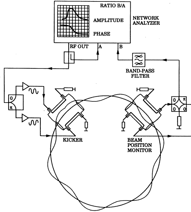
Figure 5.28: Scheme of a beam transfer function (BTF) measurement.
