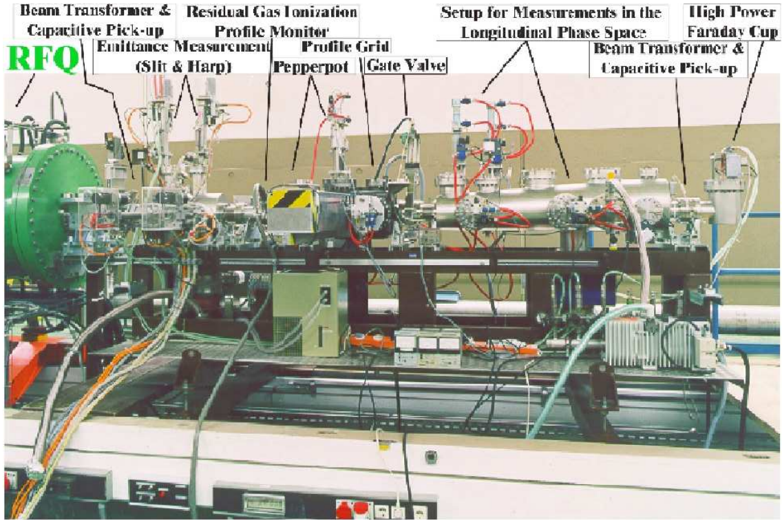
Figure 1.1: Picture of a movable test bench provided for commissioning of the new high current RFQ of GSI (green tank on the left).
