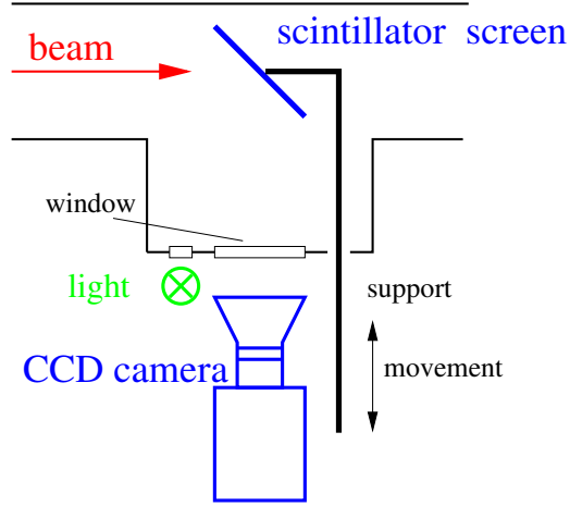
Figure 3.1: Scheme of a intercepting scintillator screen.
