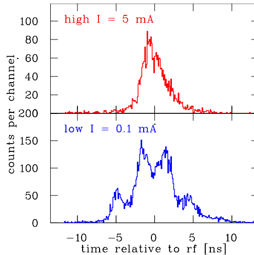
Figure 6.21: The bunch structure measured at the GSI LINAC with a 120 keV/u \text{Ar}^{1+} beam for different currents inside the RFQ [63]. The influence of the beam's space-charge to the longitudinal emittance is demonstrated by it. One rf-period is shown.
