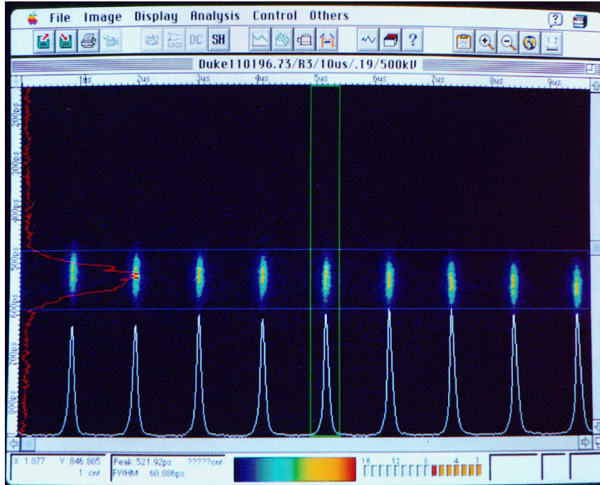
Figure 6.26: Bunch length measurement with a streak camera, using synchrotron light from a wiggler at the Duke storage ring [107]. The horizontal axis is 10 \mu\text{s} for the bunch repetition and the vertical axis is 800 \text{ ps} full scale for the bunch structure. The bunch width is 60 \text{ ps} (FWHM). A low current beam was used and the wavelength of 450 \text{ nm} is transmitted to the photo-cathode.
