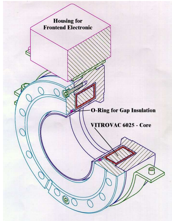
Figure 2.9: Schematic drawing for the ac current transformer used at the pulsed heavy ion LINAC at GSI.
