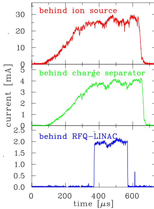
Figure 2.10: Transmission determination by ac-transformers at three different locations at the GSI LINAC using a \text{Ni}^{2+} beam from a high current source. The upper curve shows the current after the ion source where all charge states are present. The second curve is after filtering one ionic state. The third curve is the current after the first LINAC module.
