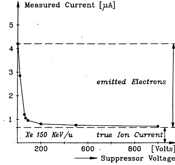
Figure 2.19: The suppression of secondary electrons in a Faraday cup as a function of the applied voltage.
