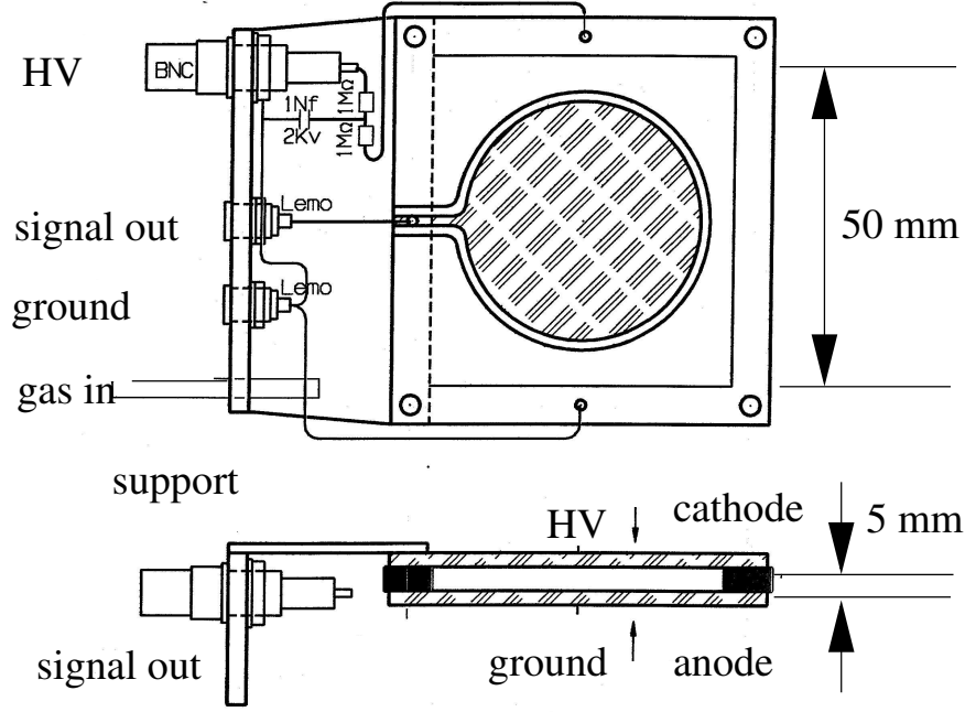
Figure 2.34: The scheme of an IC with a 5 mm active length.
