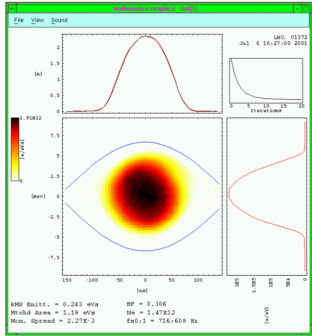
Figure 6.11: The recorded bunch shape at CERN PS using a resistive wall current monitor for 500 turns (left) and the reconstructed longitudinal phase space. The bucket size is shown in the phase space and the projections to the time axis (top) and energy (right) are displayed. From [97].
