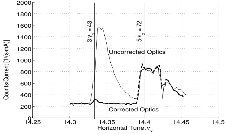
Figure 8.11: Tune scan at the ALS synchrotron light source [124]. For a fixed vertical tune, the horizontal tune is varied and the loss rate, as measured with a scintillator at a collimator is plotted. By changing the setting of some quadrupole, one resonance ( 3 \cdot \nu_x ) can be avoided.
