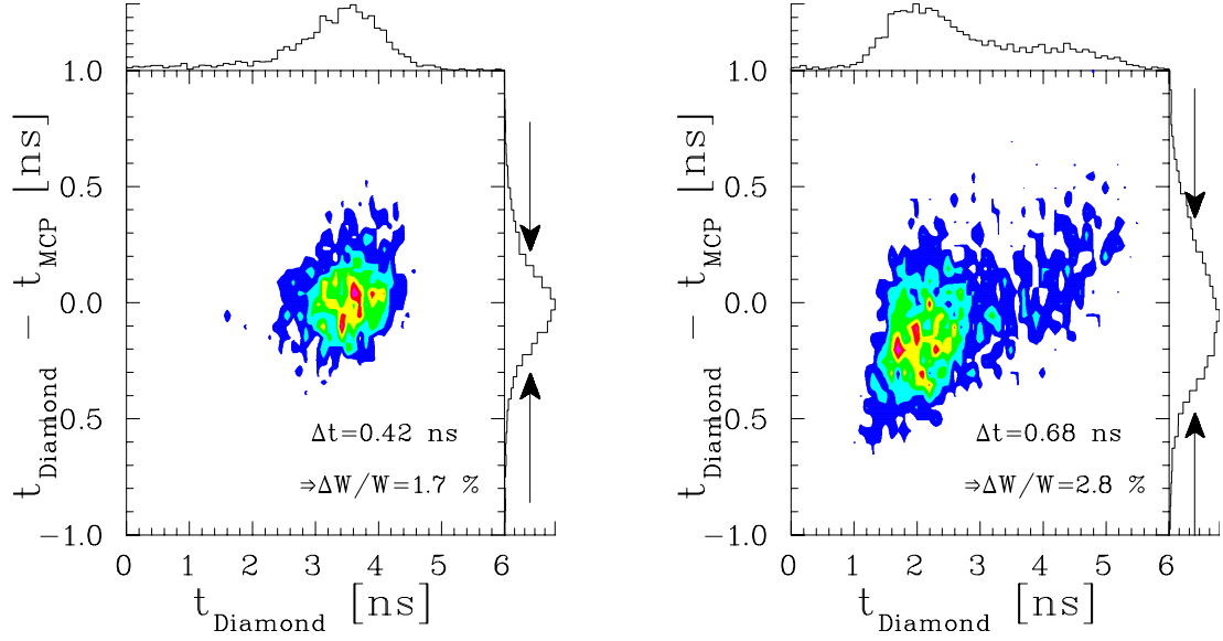
Figure 6.22: Phase space plot recorded with two detectors in coincidence at the GSI LINAC [63]. The time relative to the rf is plotted along the horizontal axis, the time difference of the individual particles on the vertical axis corresponding to the energy distribution. The low current ( I_{beam} = 0.1 mA) results are plotted left. For a high current beam ( I_{beam} = 5 mA) the emittance is asymmetrically broadened by space charge forces (right).
