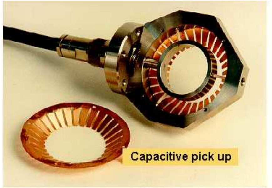
Figure 5.7: Capacitive pick-up in 50\ \Omega geometry as used for the longitudinal bunch observation at the 108 MHz GSI-LINAC. The inner diameter is 35 mm.
