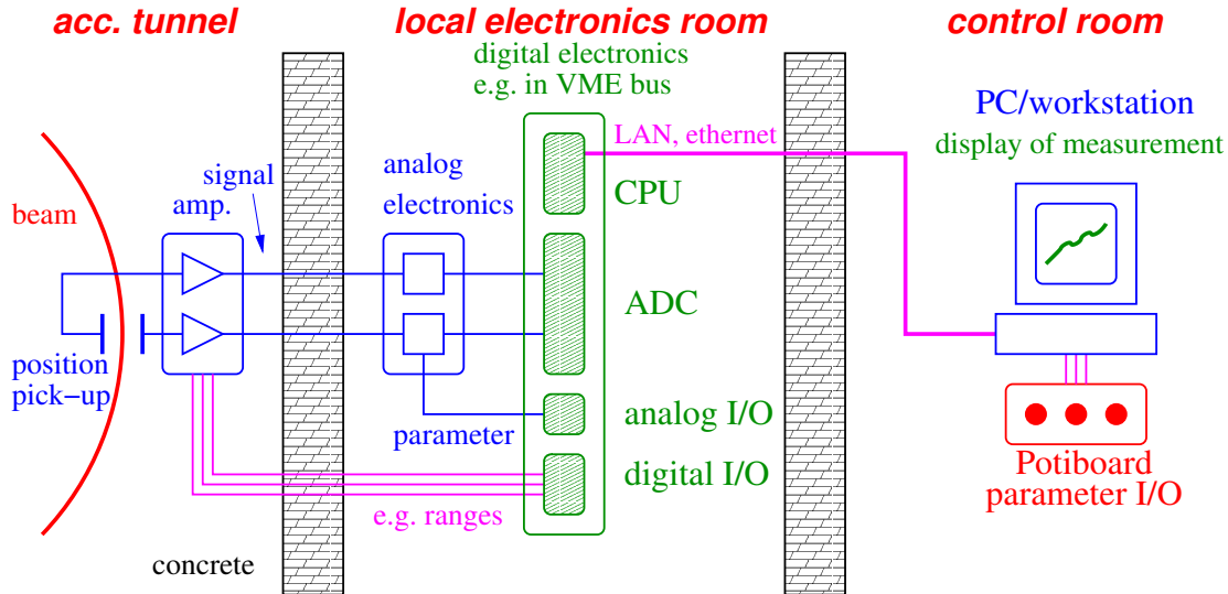
Figure 1.2: Schematics of typical beam diagnostics (here a position pick-up). The beam signal is modified by analogue electronics and digitized in a local electronics room. From the control room the parameters of the measurement, as well as for the beam can be influenced.
