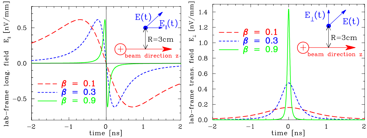
Figure 6.2: Effect of the advanced longitudinal (left) and transverse (right) electric field at an observation point R = 30 mm from the beam axis for different beam velocities. For t = 0 the closes approach is reached.
