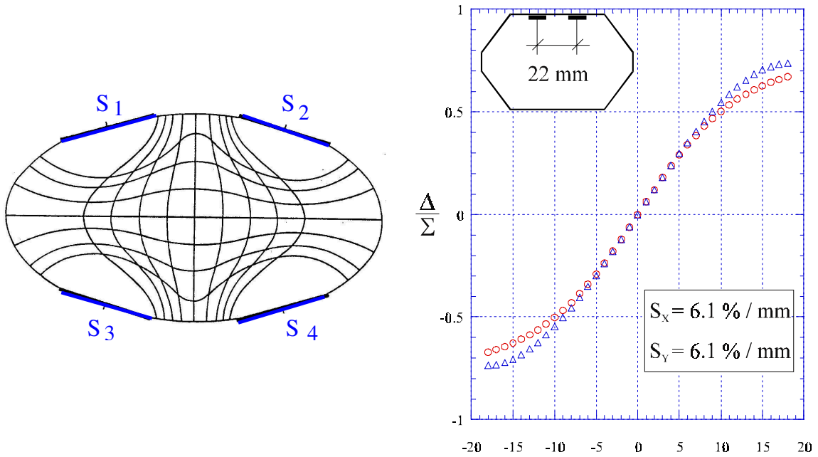
Figure 5.12: Iso-level curves for an arrangement of button pick-ups are shown on the left. On the right: The calculated accuracy for the difference voltage over the sum \Delta/\Sigma as a function of beam displacement (horizontal \circ , vertical \triangle ) for the displayed button arrangement [76].
