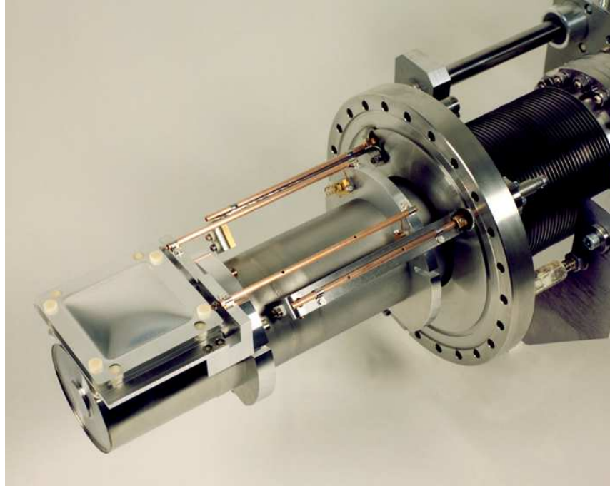
Figure 2.37: Photo of the SEM part made of 3 Al foils with thickness of 100\ \mu\text{m} of the feed-through used for slow extraction current measurements at GSI.
