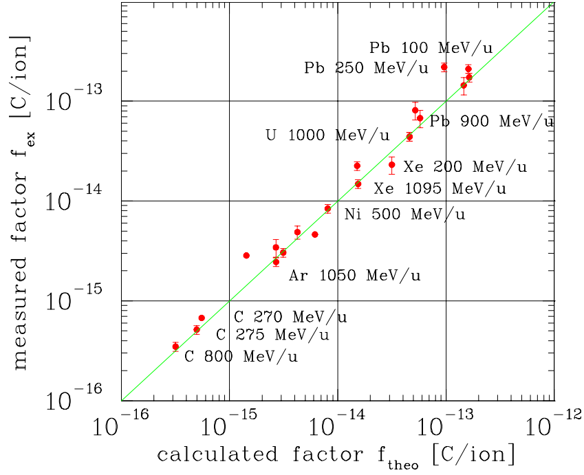
Figure 2.35: The measured calibration factor of an IC and calculated value using energy loss for various slowly extracted ion from the GSI synchrotron [17].
