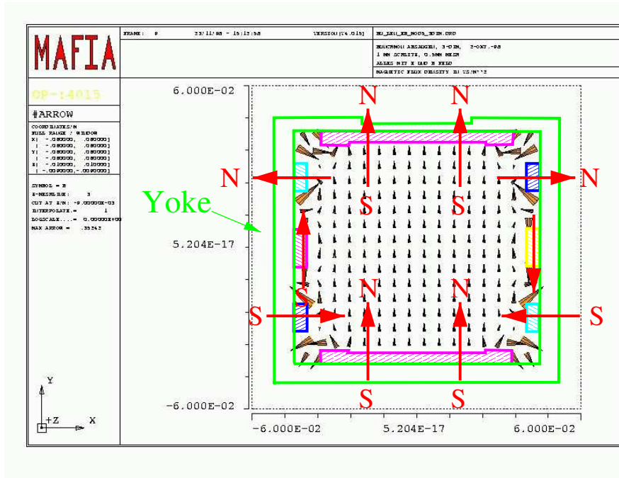
Figure 2.20: Arrangement of Co-Sm permanent magnets within the yoke and the calculated magnetic field lines. The homogeneous field strength is B \sim 0.1 T.
