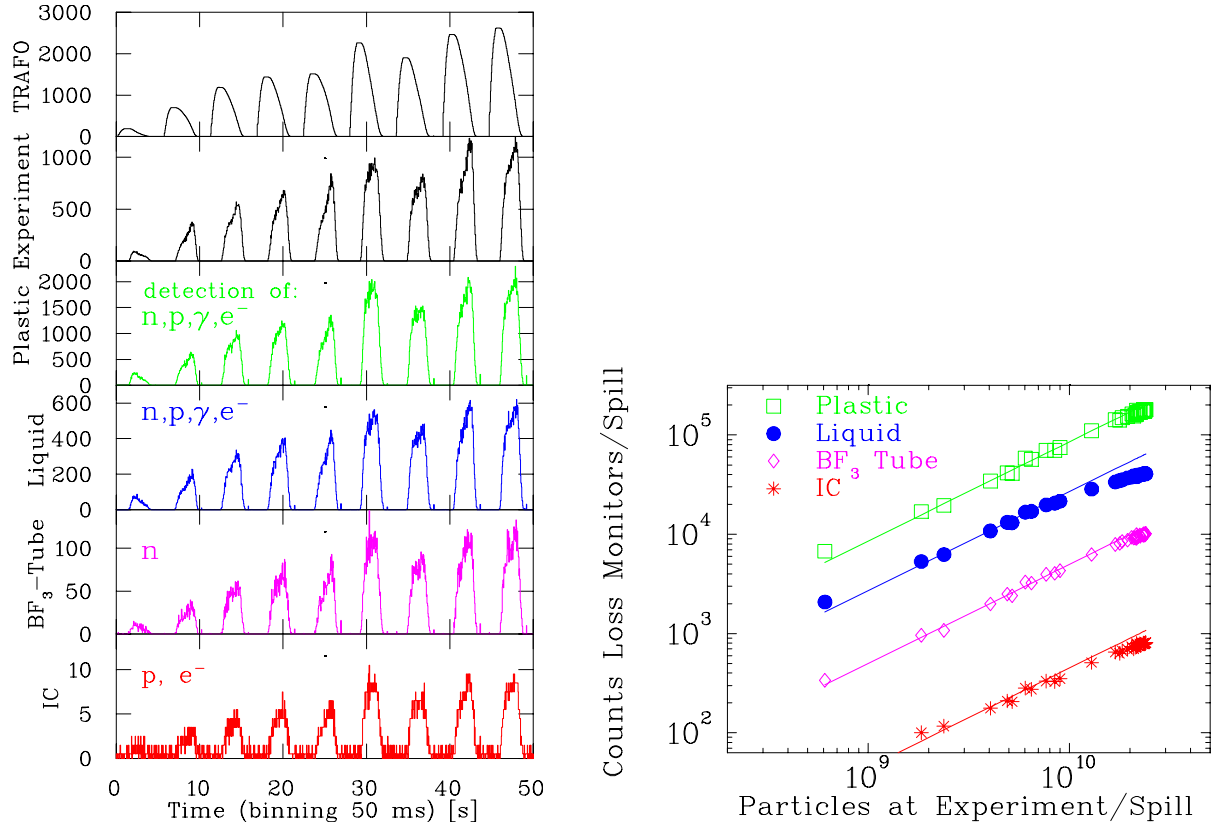
Figure 8.8: Left: Typical example from different beam loss monitors for a O^{8+} beam accelerated from 11 to 800 MeV/u with up to 4 \times 10^{10} particles per spill [118]. Right: Linearity of the loss monitors as a function of the current for the same parameters. The lines are linear fits.
