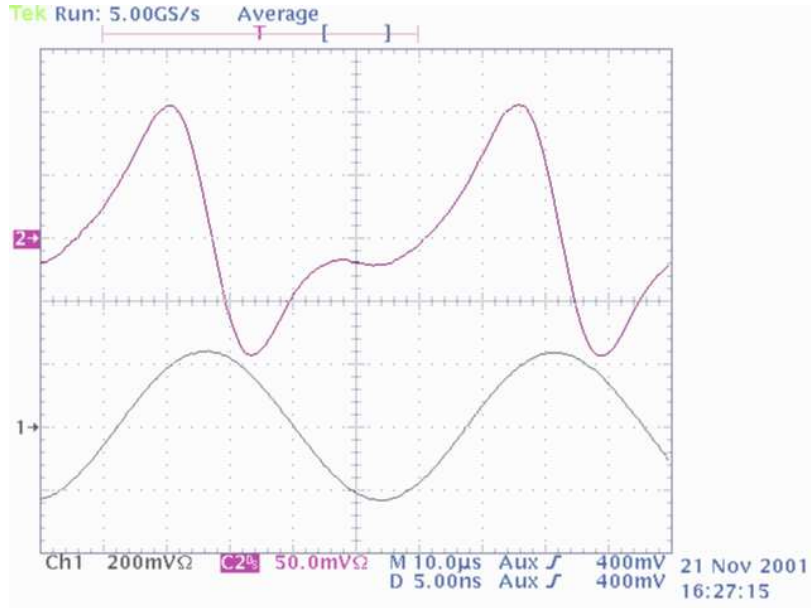
Figure 6.3: The pick-up signal from a 120 keV/u ion beam and the corresponding LINAC module frequency for the determination of the bunch position.
