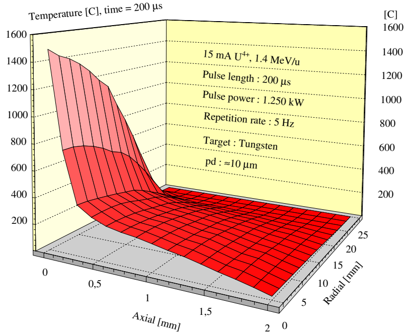
Figure 2.25: A 1.4 MeV/u \text{U}^{4+} beam of 15 mA electrical current and 0.2 ms pulse length hitting a cooled cylindrical Faraday cup. The distribution of the temperature is calculated by finite element method.
