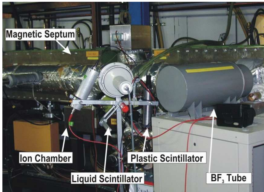
Figure 8.2: The tested beam loss detectors installed at the extraction from the GSI heavy ion synchrotron [118].
