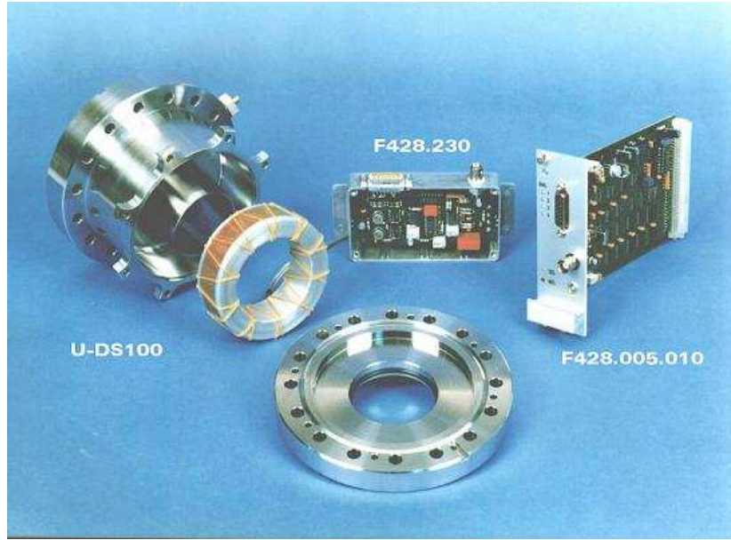
Figure 2.8: Photo of an ac-current transformer used at the pulsed heavy ion LINAC at GSI. The torus with the differential winding is shown left, the used electronic modules at the right.
