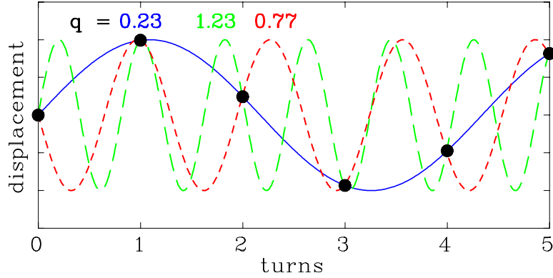
Figure 5.25: Schematic of the tune measurement for six subsequent turns determined with one pick-up, together with the three lowest frequency fits.
