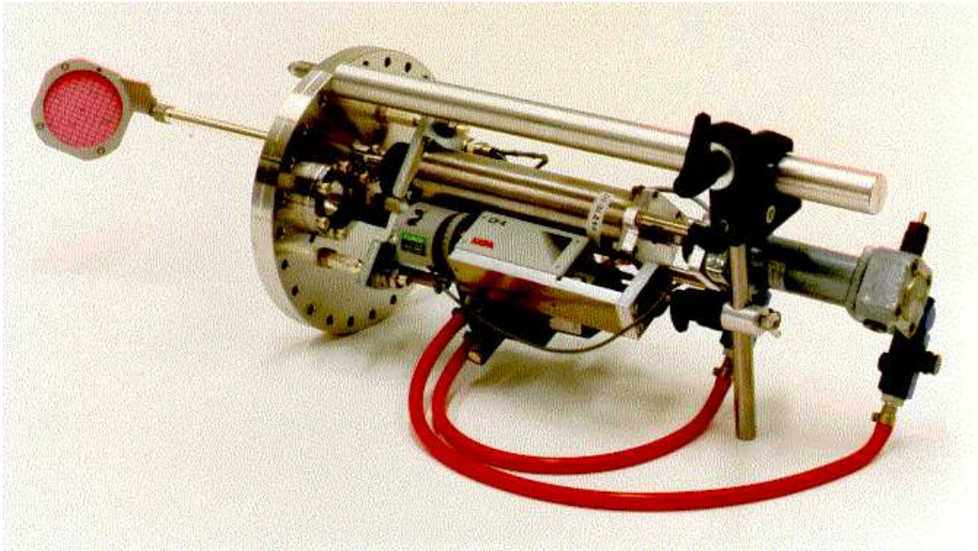
Figure 3.2: A Chromolux scintillation screen of Ø70 mm mounted on a Ø200 mm feed-through including the CCD camera.
