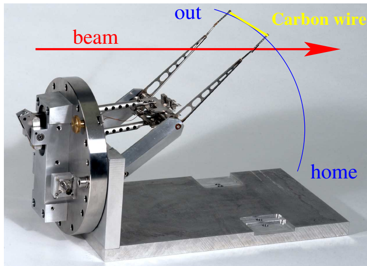
Figure 3.10: Pendulum scanner or 'flying wire' used at CERN synchrotron [26].
