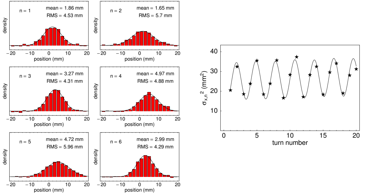
Figure 3.9: Profile measurement for a mismatched injection into the CERN PS synchrotron for the first n = 1 \dots 6 turns and the fitted square of the beam width as a function of time, from [32].
