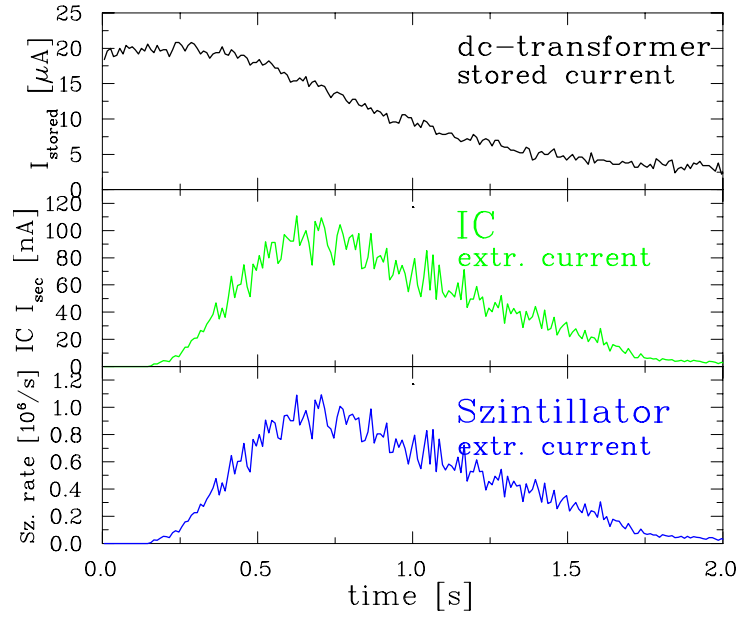
Figure 2.32: The extracted current measured with an IC (middle, given in nA for the secondary current) and a scintillator (bottom, given in particles per second) as compared to the current inside the GSI synchrotron determined by dc-transformer (top, given in \mu\text{A} ) for one extraction of a 250 MeV/u ^{208}\text{Pb}^{67+} beam with a total amount of 10^6 particles.
