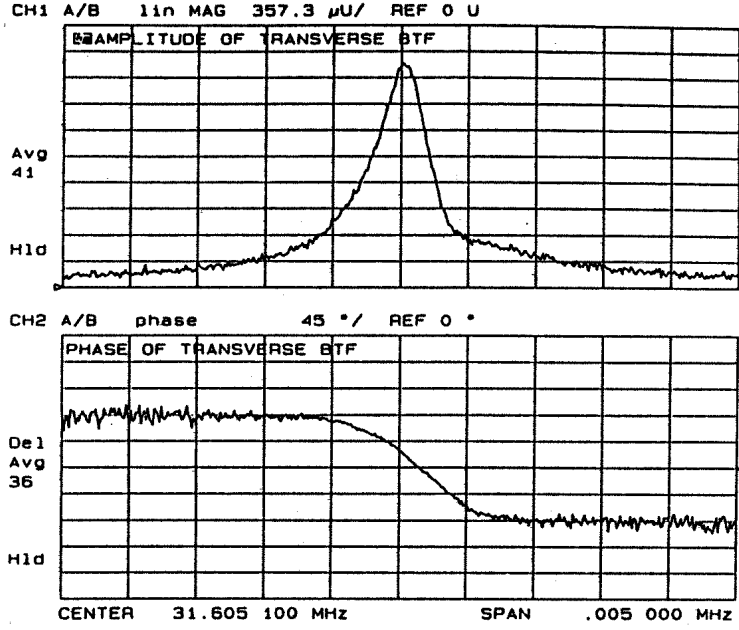
Figure 5.29: BTF measurement with a cooled ion beam at the GSI storage ring ESR, recorded with a scan around the 22 nd harmonic. The amplitude on a linear scale (top) and the phase with 45°/div (bottom) is shown.
