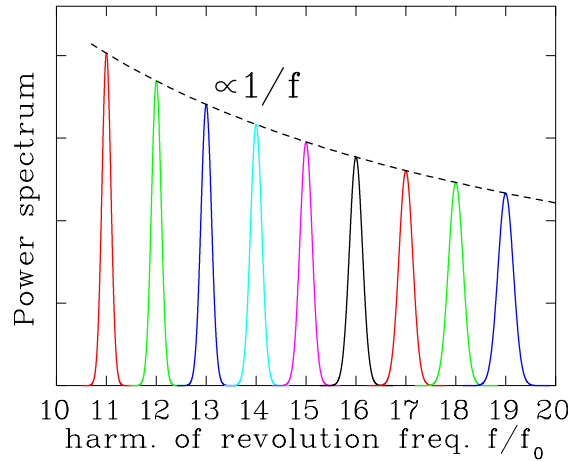
Figure 7.3: Hypothetical longitudinal Schottky lines for a Gaussian momentum distribution with \Delta p/p = 1\% and an artificial small value of \eta = 0.005 . The different peaks correspond to the different harmonics.
