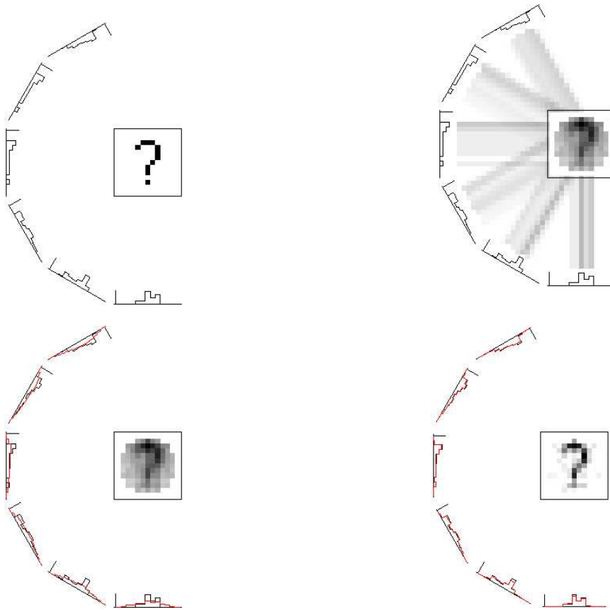
Figure 6.10: Schematic plots for the tomographic reconstruction technique [96]. The original 2 dimensional image and the 1-dim projections are shown to the left. A first back projection is shown top right. The first iteration step for the generation of the differences in the projected data is plotted bottom left. After \sim 50 iterations, the original image can be reconstructed.
