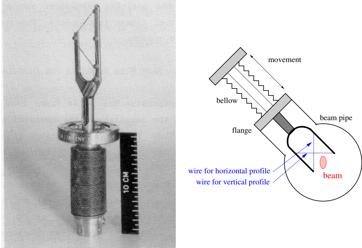
Figure 3.12: Linear scanner used at CERN [29].
