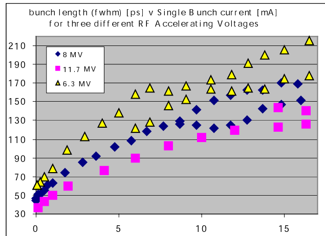
Figure 6.27: Example of the use of a streak camera at the synchrotron light facility ESRF [104]: The bunch-length is recorded as a function of the current per bunch for different accelerating voltages.
