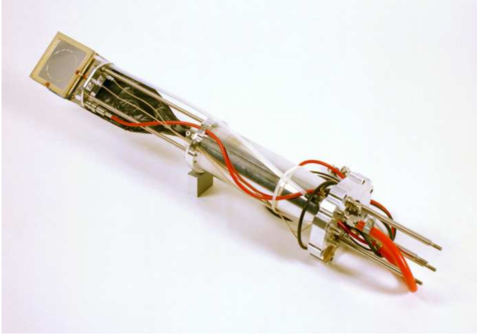
Figure 2.30: The hardware of the scintillators (wrapped in black tape) and the IC installed at GSI.
