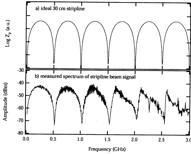
Figure 5.18: Calculated transfer impedance of an ideal 30 cm stripline (a) and and a measurement (b) with a spectrum analyzer for a single bunch signal [67]. The frequency range is 0 to 3 GHz.
