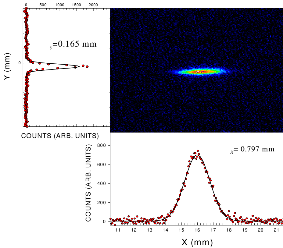
Figure 3.31: Image of the electron beam in the APS accumulator ring (Argonne National Lab.) by a synchrotron radiation monitor [56].
