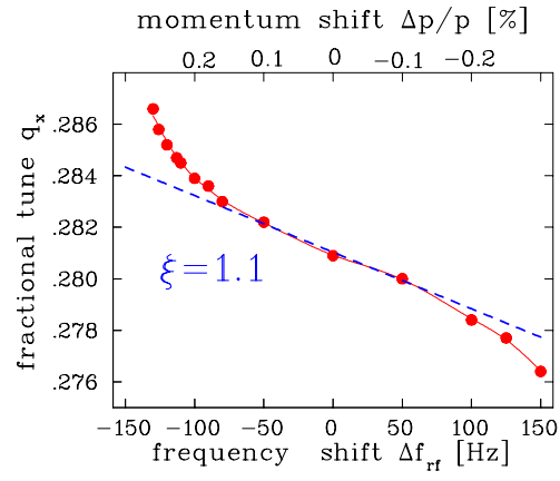
Figure 5.32: Measurement of the chromaticity at LEP. The horizontal tune is determined for different setting of the acceleration frequency and therefore of the momentum of the circulating beam. The chromaticity is fitted through the linear part of the data [91].
