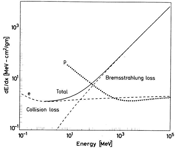
Figure 2.22: The energy loss of electrons in copper for collision and radiation losses [10]. For comparison the loss of protons are also shown.
