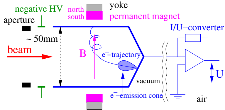
Figure 2.17: Scheme of an uncooled Faraday cup with magnetic and electric secondary electron suppression.
