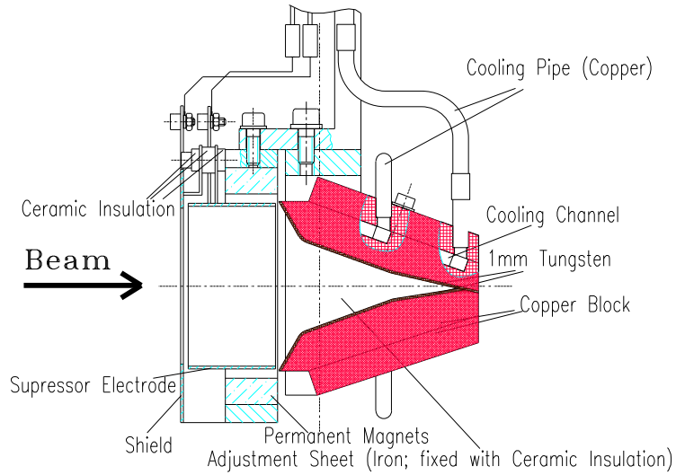
Figure 2.26: A Faraday cup and beam stopper of high intensity beams as installed at the high current LINAC at GSI. The opening of the cup is \varnothing 50 mm
