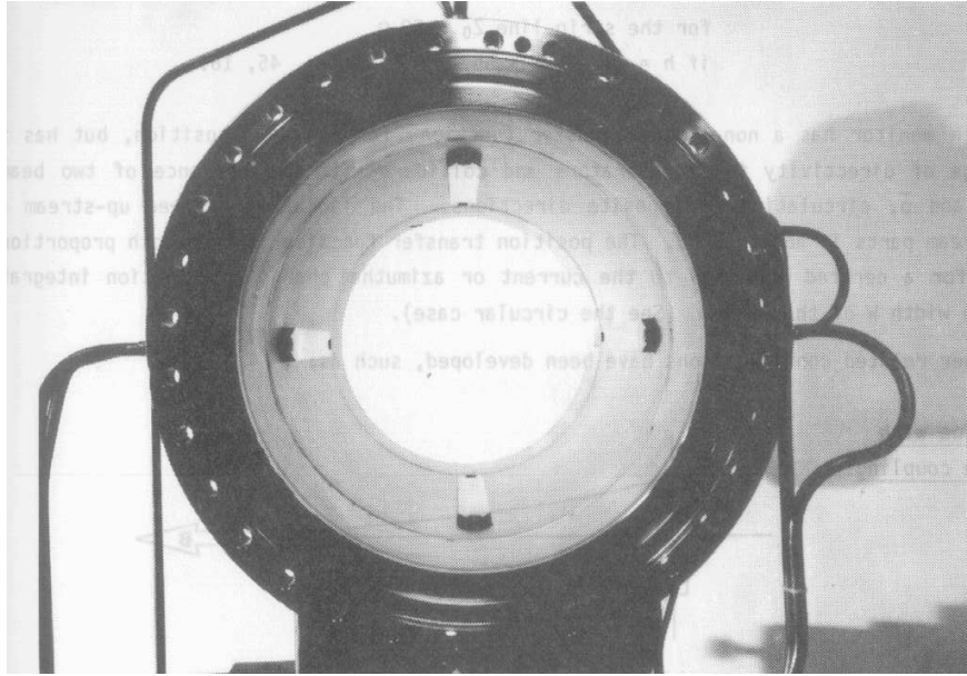
Figure 5.19: Photo of a stripline pick-up at the CERN SPS, from [73].
