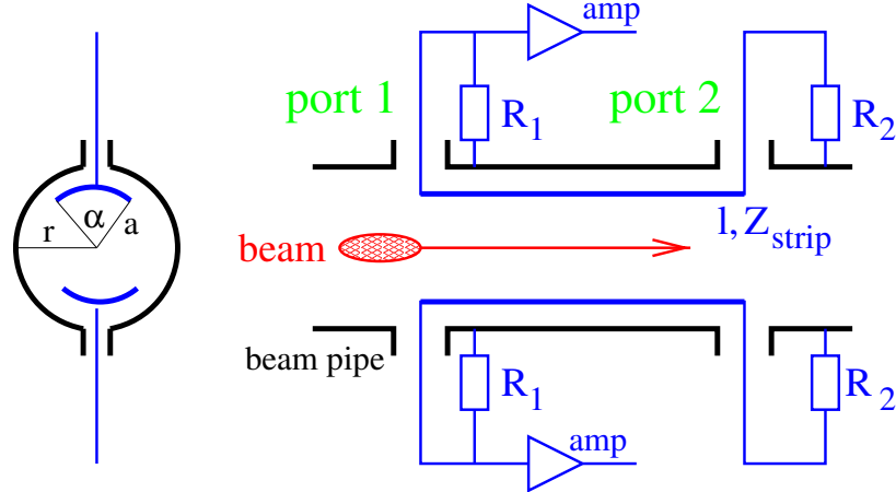
Figure 5.16: Scheme of a stripline pick-up.
