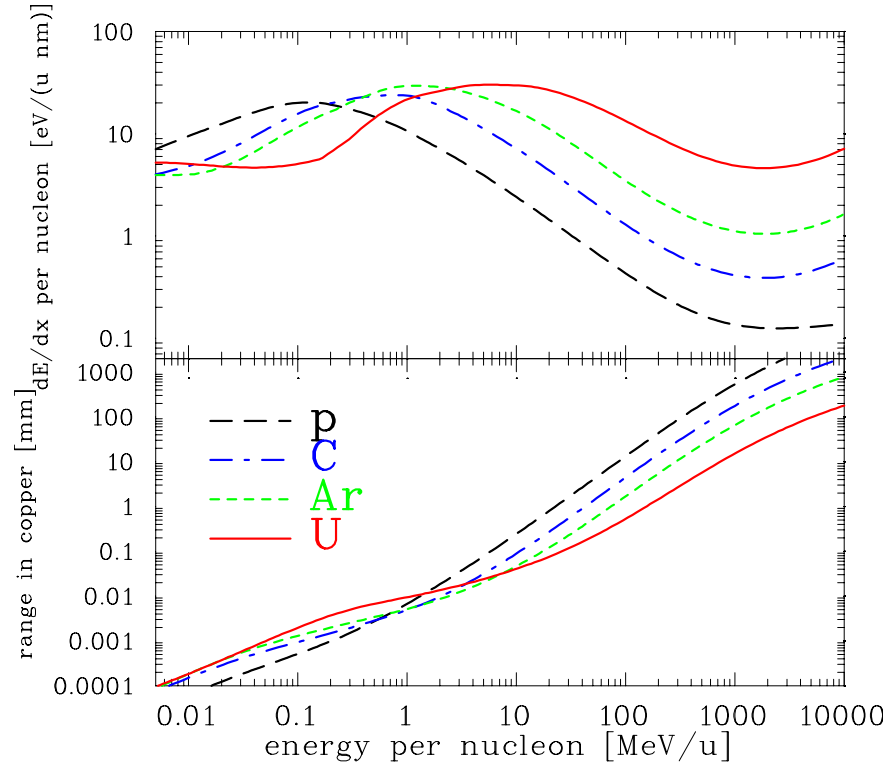
Figure 2.21: The energy loss per nucleon at the surface and the range in copper as a function of the kinetic energy for several ions. The energy range is plotted from 5 keV/u to 10 GeV/u and the range from 100 nm to 1m. The calculation of the electronic and nuclear stopping uses SRIM [13].
