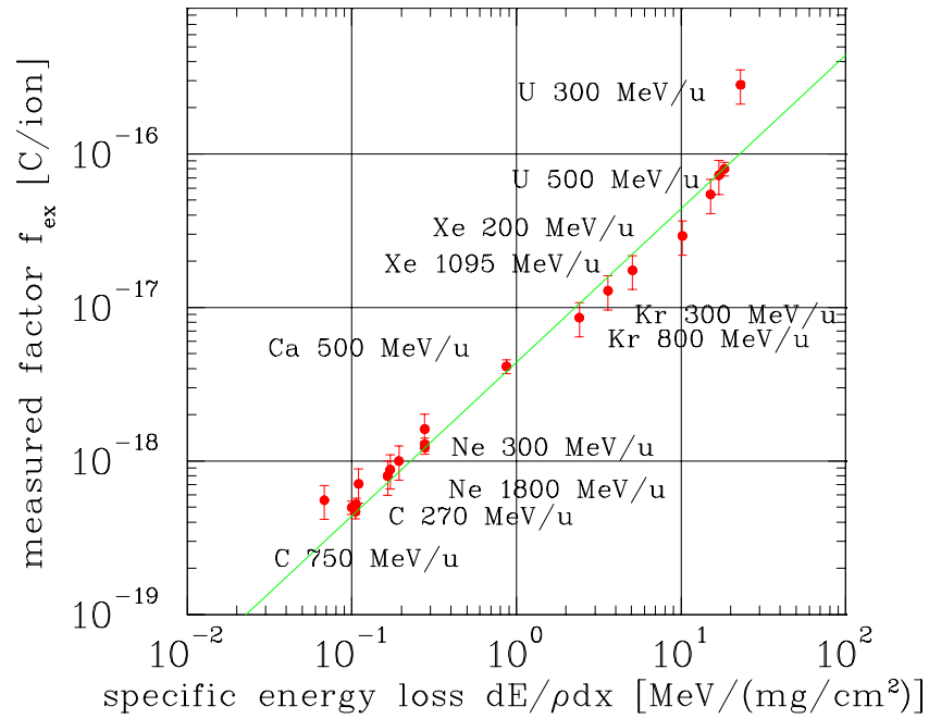
Figure 2.38: The measured calibration factor of a SEM and calculated value using energy loss and a fitted value of Y = 27.4\ e^-/(\text{MeV}/\text{mg}/\text{cm}^2) for various slowly extracted ion from the GSI synchrotron [17].
