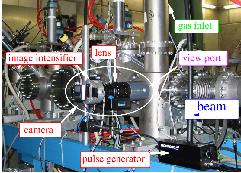
Figure 3.23: The installation of the intensified camera at the target location for test at GSI.
