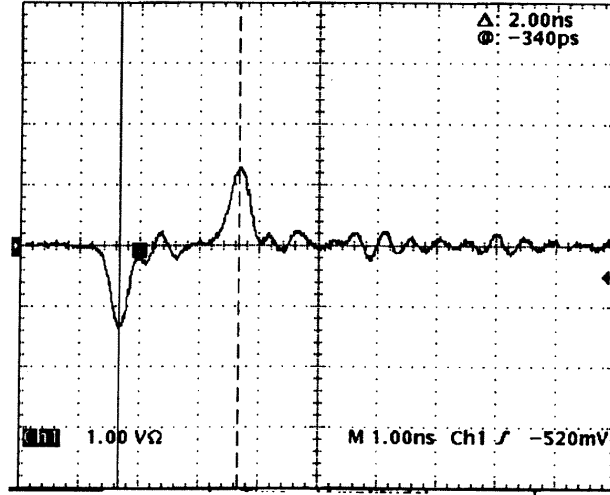
Figure 5.17: Single shot signal from from a 30 cm stripline pick-up recorded at the ALS synchrotron light facility for a single bunch with 1 ns/div [67].
