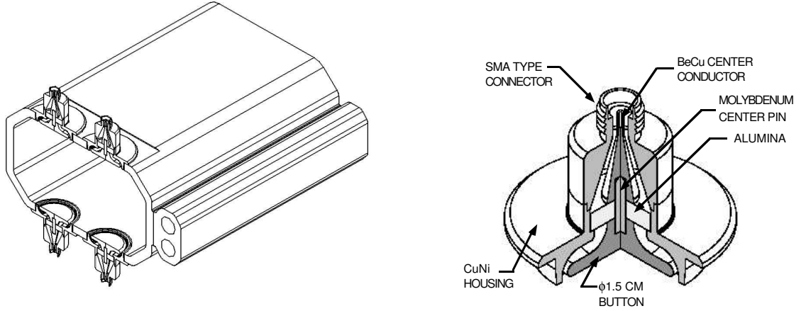
Figure 5.11: Drawing of a typical button pick-up for an electron accelerator; from the electron-positron collider PEP [74].
