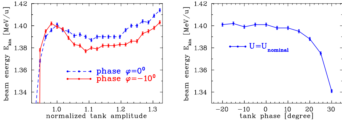
Figure 6.6: The output energy of the GSI-LINAC as a function of the applied rf-amplitude inside the tank (left) and phase for the nominal amplitude (right). The required energy of this module is 1.400 MeV/u. The distance between the pick-ups is L = 1.97 m with N = 4 bunches between.
