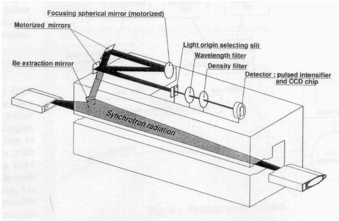
Figure 3.30: The synchrotron radiation profile monitor at LEP. The optical system is installed close to the 23 m long dipole magnet with bending radius of 3100 m, from [55]
