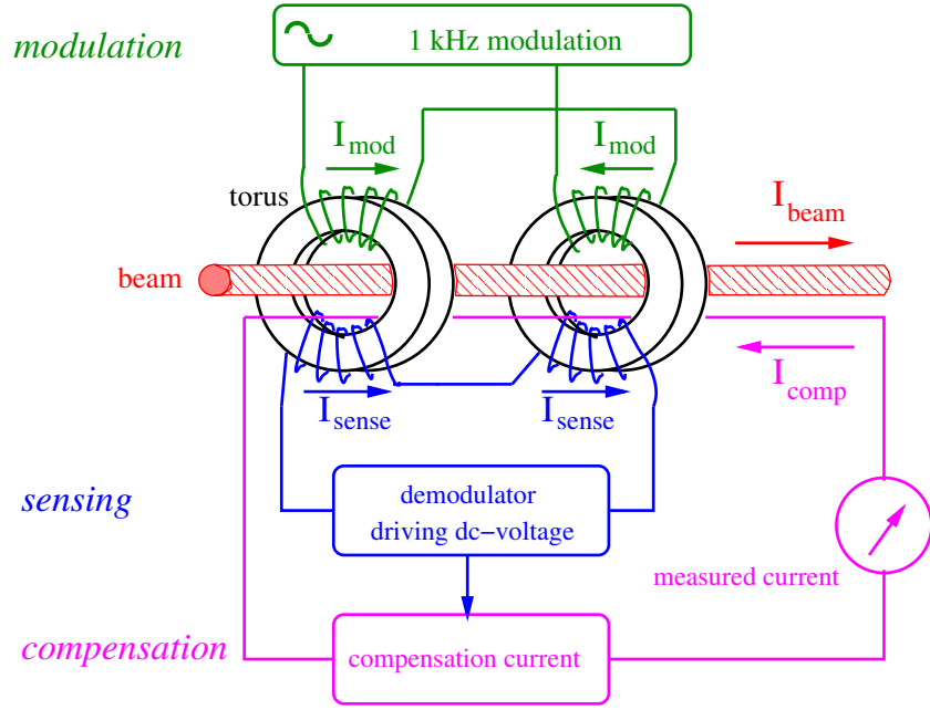
Figure 2.12: Schematics of a dc-transformer, see text.
