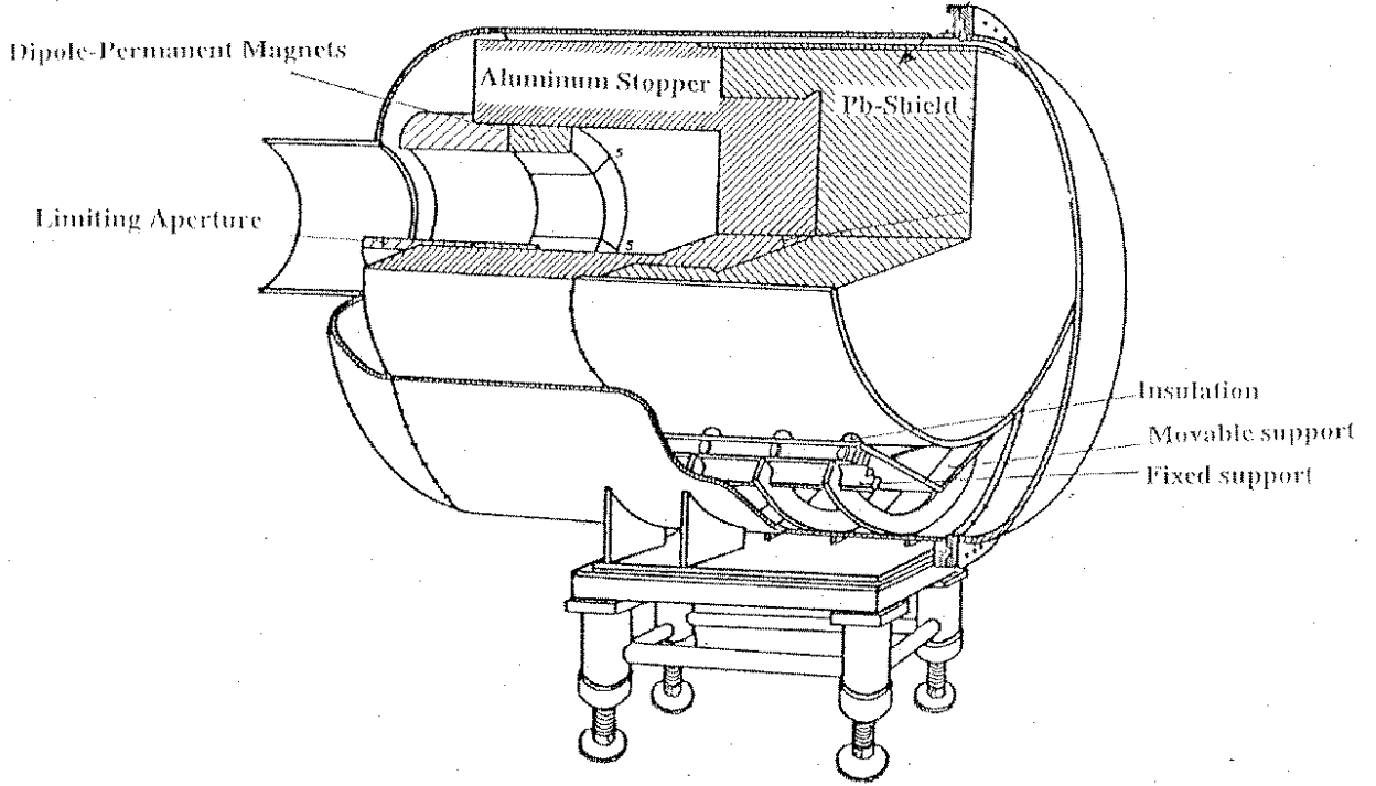
Figure 2.23: A drawing of a cup used for 60 MeV electrons.
