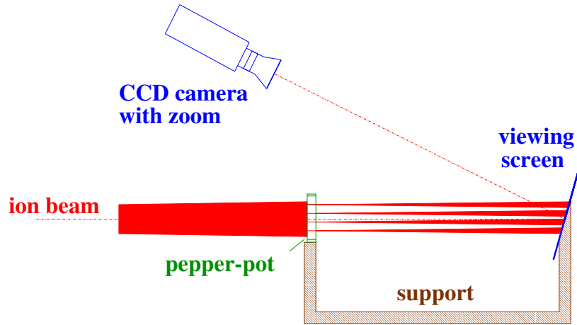
Figure 4.4: Scheme of a pepper-pot emittance measurement device.
