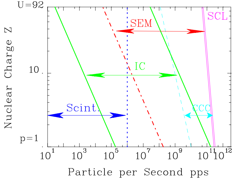
Figure 2.28: Overview of the different detector systems used for slow extraction at the GSI synchrotron. The numbers are given for the different ions with an kinetic energy of 1 GeV/u, extracted within 1 s and a spot size of 1 cm 2 . With a scintillator up to 10 6 particles can be counted. The lower limit of the IC and SEM correspond to a secondary current of 1 pA, the upper threshold of the IC is 30 Gray/s. The CCC (cryogenic current comparator) measures the magnetic field. SCL means the incoherent space-charge limit of the synchrotron at injection energy.
