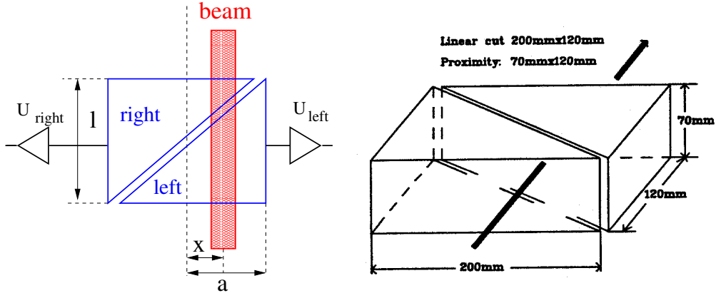
Figure 5.13: Scheme of the position measurement using the so-called linear cut and an example of an electrode arrangement for the horizontal plane.
