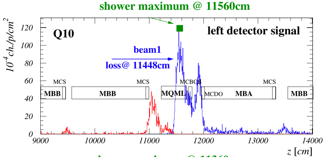
Figure 8.9: Simulation of a secondary particle distribution (hadron shower) due to a proton loss inside a quadrupole for the LHC and 7 TeV protons [122]. The maximum of the shower is about 1 m from the loss point.
