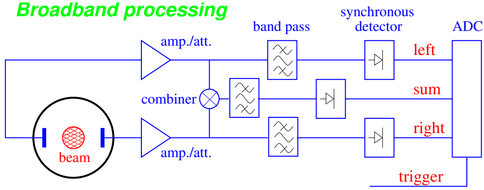
Figure 5.20: Schematic of signal analysis for a broadband treatment.
