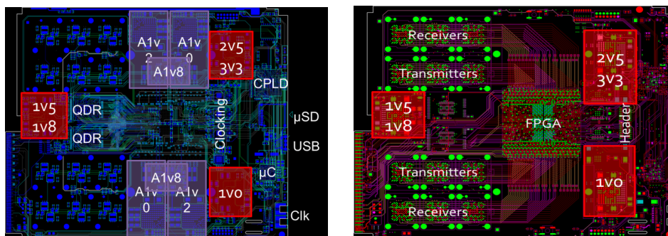
Figure 4. Distribution of power supplies on the MP7 processor board: left shows the bottom surface of the board and right shows the top surface. The red boxes indicate the bulk supplies based on the Linear LTM4620 [4] and LTM4628 [5] regulators and the purple boxes indicate the “analogue” power supplies for the multi-gigabit transceivers.
