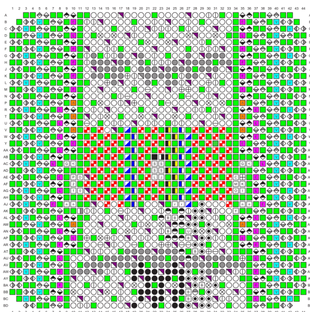
Figure 2. Pin-out of the XC7VX690T FPGA in a FFG1927 pin package. Pins coloured green are ground pins, those in other colours are power-supply pins and those in grey-scale are I/O pins: approximately half the pins are dedicated to powering the chip.
