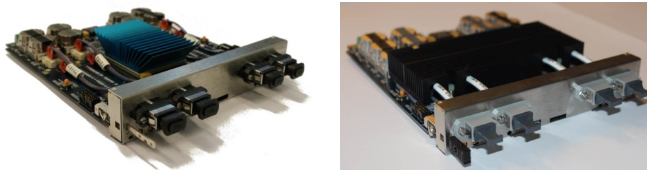
Figure 6. Left, the initial prototype MP7 used an off-the-shelf heatsink and, right, the custom-designed heatsink used for final production.
