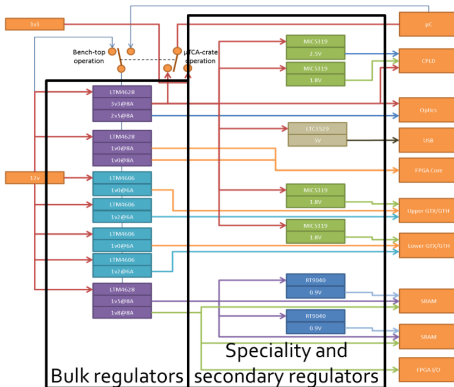
Figure 3. Power architecture used on the initial design of the MP7 processor card. A two-step architecture is used: a bulk step-down and a fine step-down.
