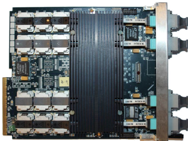
Figure 1. The Imperial MP7 processor. The MP7 is based on the Xilinx Virtex-7 FPGA (under the custom-designed heatsink) and Avago MiniPOD optical modules. The MP7 provides 72+72 optical serial links capable of operating at over 10Gbps giving a total bandwidth of 0.75+0.75Tbps.
