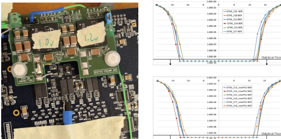
Figure 5. Left, one of the test-boards for evaluating the performance of alternative transceiver power supplies. The board shown here is the LTM4601 design chosen for the final design. The plots on the right show the bath-tub curves for a selection of the 10Gbps links using the LTM4606 (top) and LTM4601 (bottom) designs. The bit-error rate of both designs hits the statistical floor at the centre of the eye.
