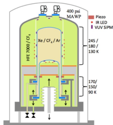
LAr Bubble Chamber
