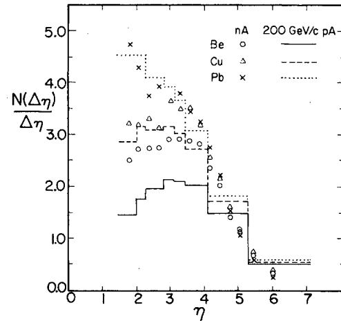
FIG. 11. Comparison of pseudorapidity distributions for \eta \gtrsim 1.5 for 200-GeV/c pA interactions from this experiment (histogram) and nA interactions from Ref. 22 (points).
