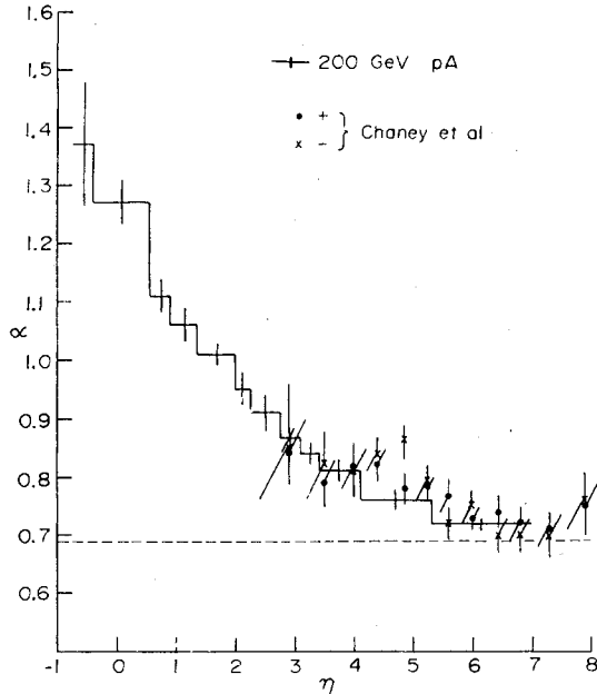
FIG. 10. Exponent \alpha , where the inclusive cross section \sigma(\Delta\eta)/\Delta\eta is assumed to follow the form A\alpha^{\eta} . The form A^{0.69} has been assumed for the total inelastic cross section so that data from this experiment (histogram) can be compared directly with data from Ref. 21. (Points refer to positively charged secondaries, crosses refer to negatives.)
