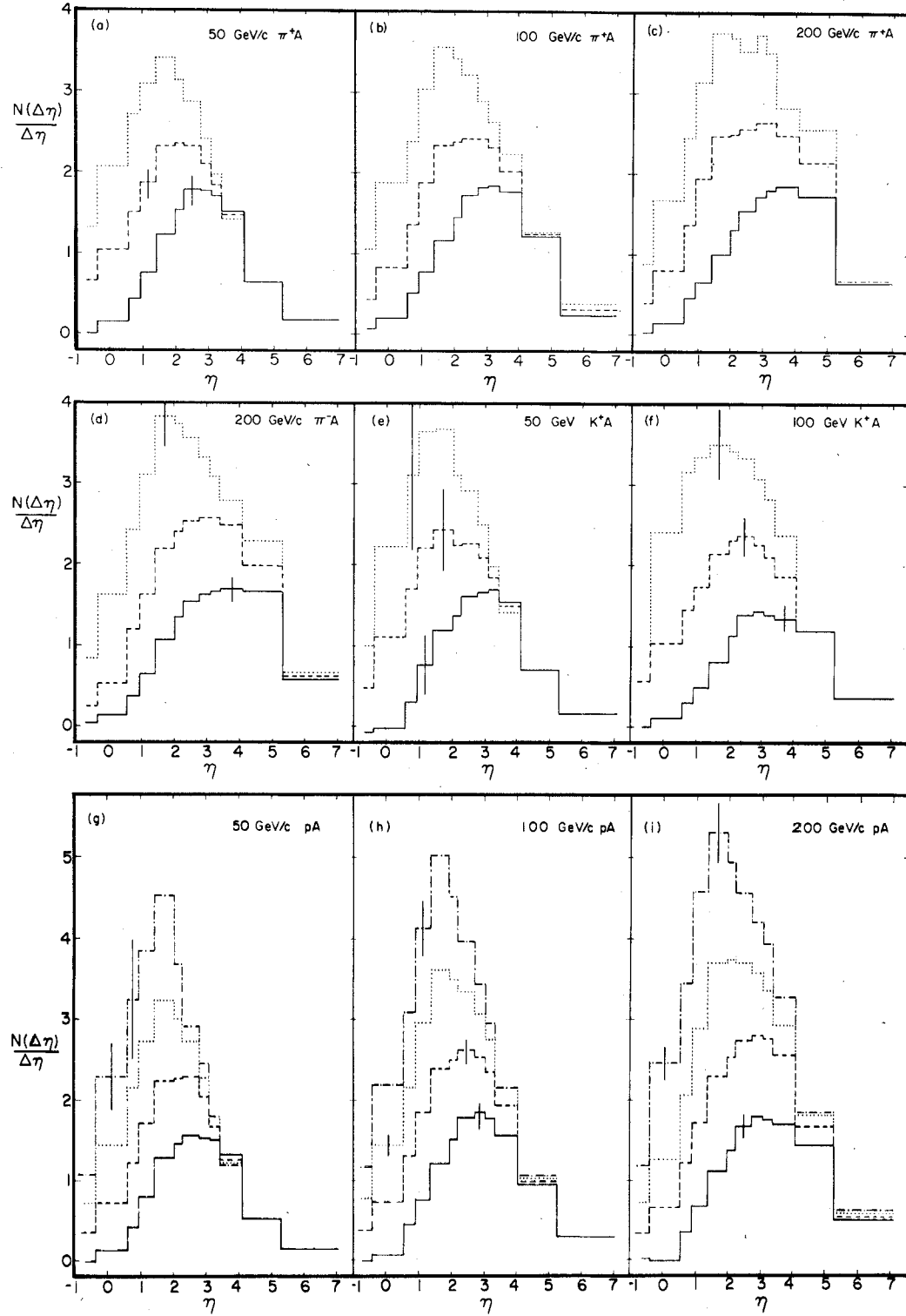
FIG. 22. Nuclear-thickness variation of pseudorapidity distributions of charged secondaries. The solid line, broken line, dotted line, and dot-dashed line refer to results at \bar{p}=1, 2, 3 , and 4 , respectively. Typical errors are shown.
