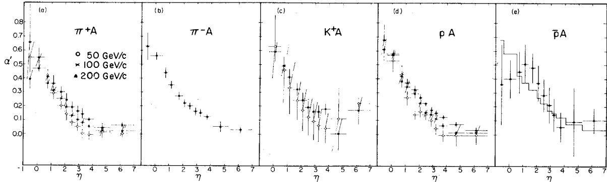
FIG. 17. Exponent \alpha' , where the normalized inclusive cross section 1/\sigma_{tot} \sigma(\Delta\eta)/\Delta\eta is assumed to follow the form A\alpha'(\eta) . \pi^+ , \pi^- , K^+ , p , and \bar{p} induced data are shown in (a), (b), (c), (d), and (e), respectively. p induced data are superimposed on \bar{p} data for comparison.
