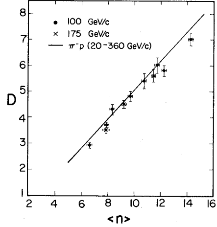
FIG. 16. Dispersion vs mean of multiplicity distribution for \pi A interactions at 100 and 175 GeV/c. Data are from Tables III and IV. For comparison, the best fit to \pi p data from Ref. 25 is also shown.
