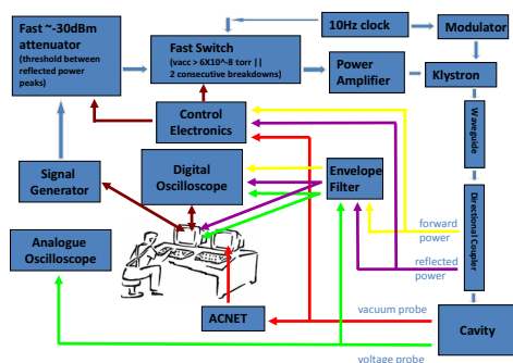
Figure 2: Schematic of the new experimental setup showing the hardware used and the signals used to control the power input to the cavity.
