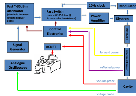
Figure 1: Schematic of the old experimental setup showing the hardware used and the signals used to monitor the cavity.
