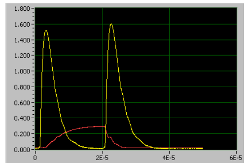
Figure 3: Reflected power (yellow) and pickup probe (red) signal after the envelope filter has been applied.
