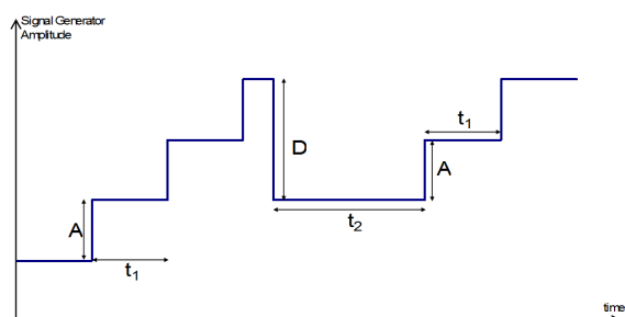
Figure 5: Graph showing how the ACS might vary the signal generator amplitude as a function of time. A is the fixed increment of the amplitude and t_1 is the time between amplitude increments. D is the amplitude decrement and t_2 is the time interval before the next increment, both of which are determined by the breakdown condition that was exceeded.
