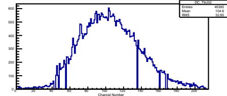
Clusters in Channel TKU S4 P2
