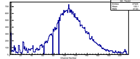
Clusters in Channel TKU S3 P2
