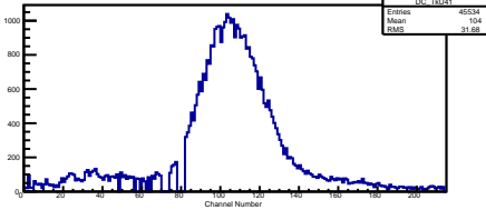
Clusters in Channel TKU S5 P1
