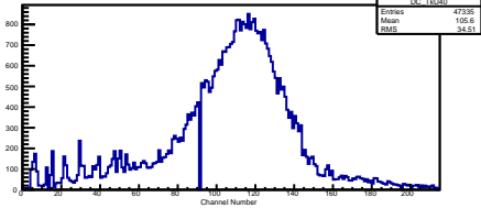
Clusters in Channel TKU S5 P0
