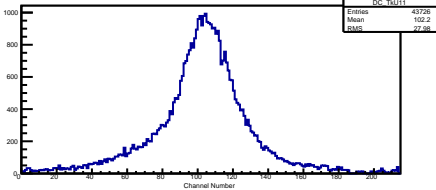
Clusters in Channel TKU S2 P1
