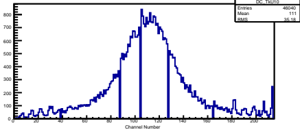
Clusters in Channel TKU S2 P0
