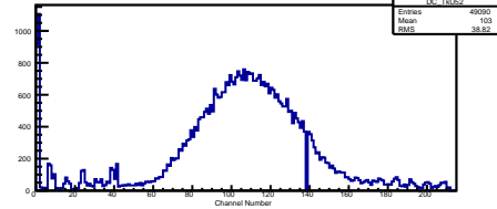
Clusters in Channel TKU S5 P2
