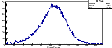
Clusters in Channel TKU S3 P1
