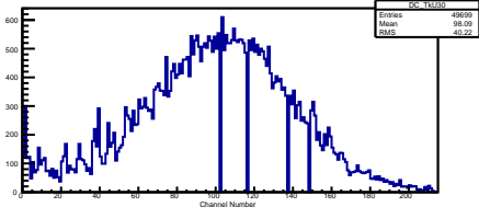
Clusters in Channel TKU S4 P0
