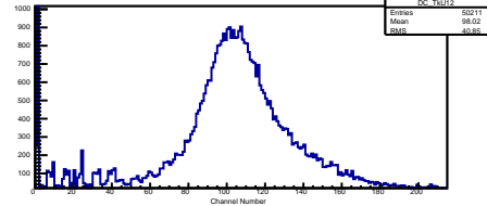
Clusters in Channel TKU S2 P2
