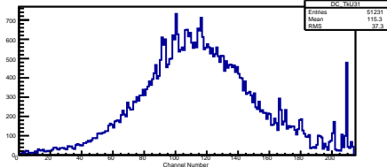
Clusters in Channel TKU S4 P1
