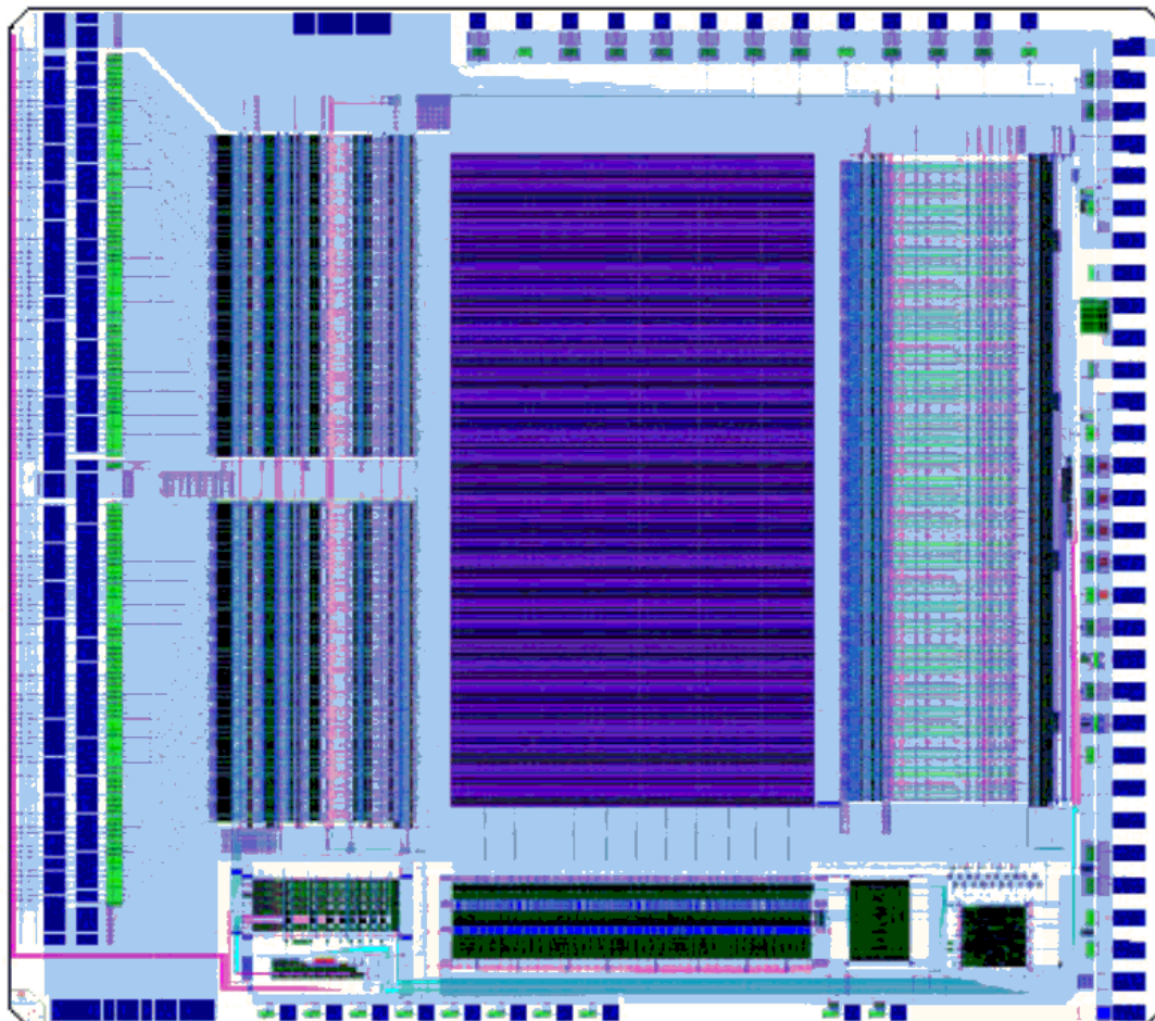
Figure 1: APV25 Layout
